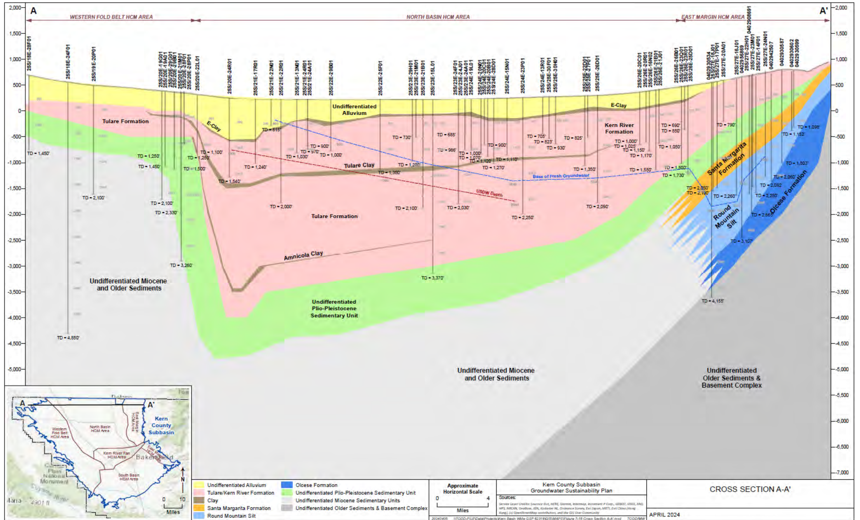
Figure 7-15. Cross Section A-A'
