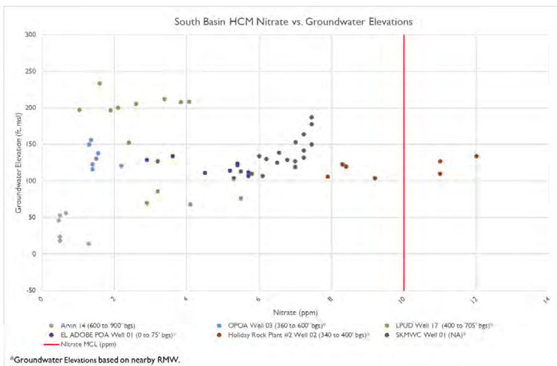
Figure 8-39. South Basin HCM Nitrate vs. Groundwater Elevations
