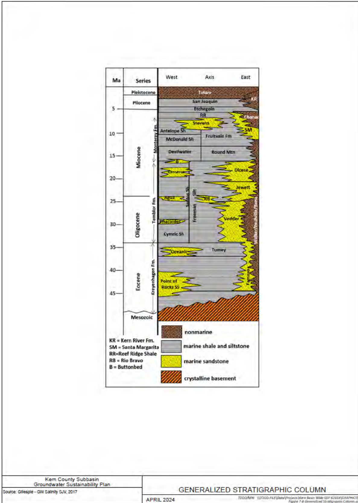
Figure 7-8. General Stratigraphic Column
