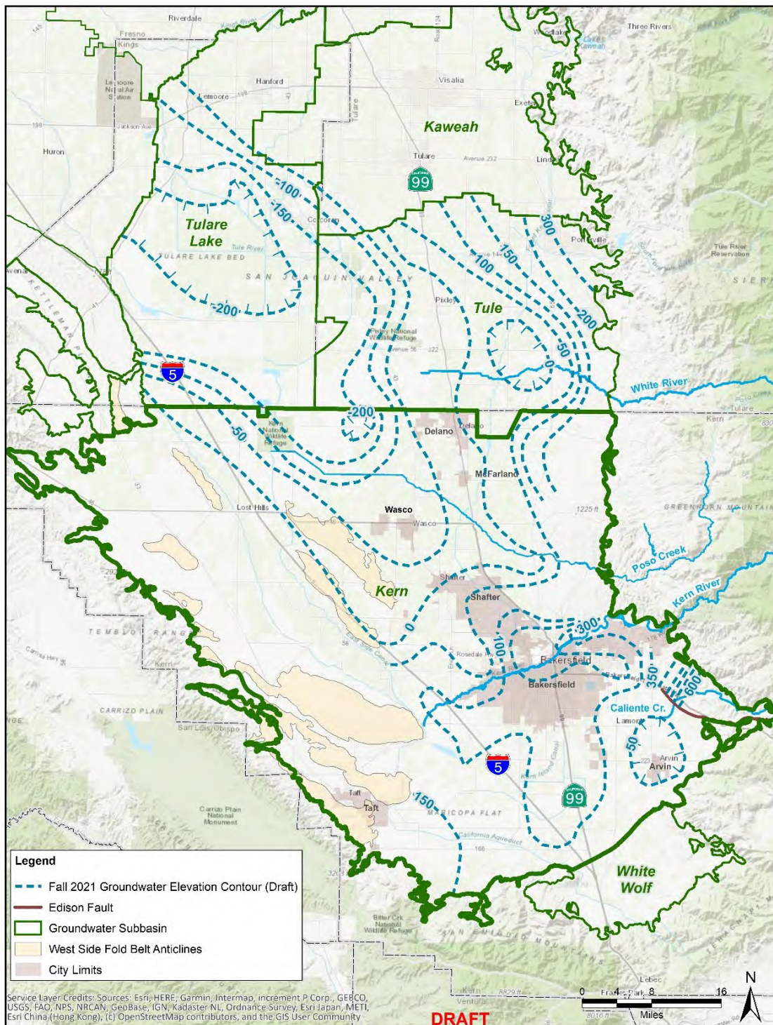
Kern County Subbasin Groundwater Sustainability Plan FIGURE 8-6 REGIONAL GROUNDWATER ELEVATION MAP – LOWER AQUIFER ZONE Sources: MAY 2024 I:\DD\AW - \Projects\Kern Basin Wide GSP 6.2.18\GIS\MAPS\ Figure 8-6 Regional Groundwater Elevation Map.mxd - 20240502
